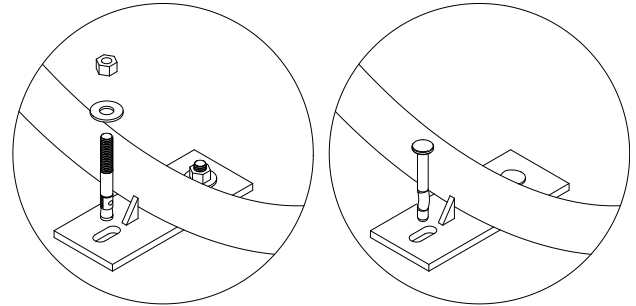
Wedge Anchor
